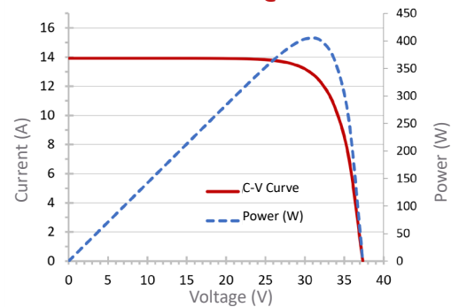
C-V and Power Curve @ STC
