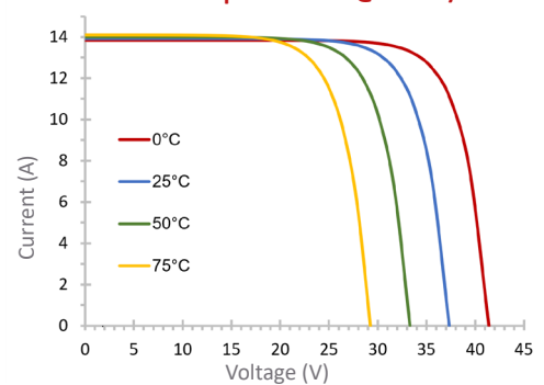
C-V and Temperature °C @ 100W/m 2
