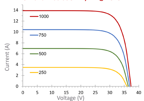
C-V and Irradiation W/m 2 @ 25°C
