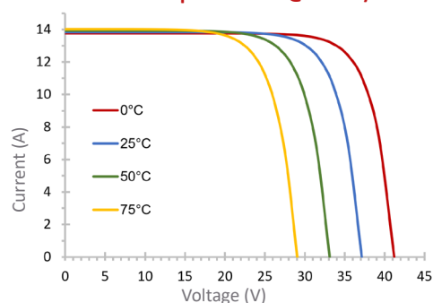
C-V and Temperature °C @ 100W/m 2
