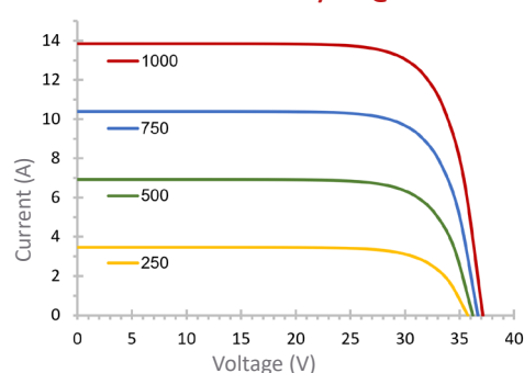
C-V and Irradiation W/m 2 @ 25°C
