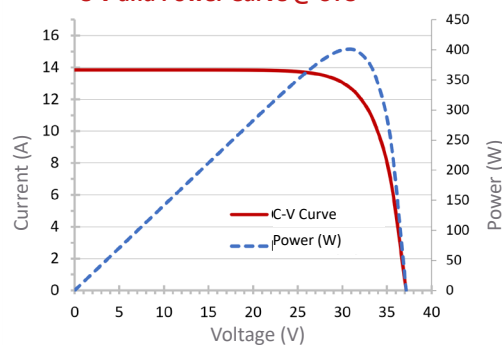
C-V and Power Curve @ STC
